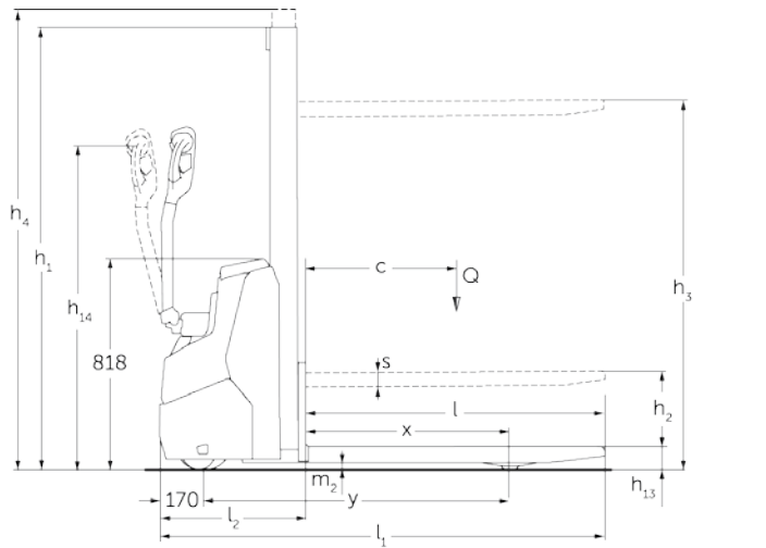
EJC 110i (Fork Over)
